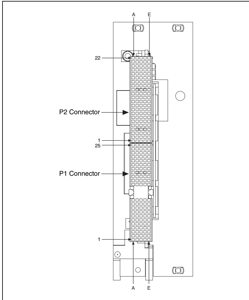
Figure C-6. PXI Connector Locations and Pinouts
