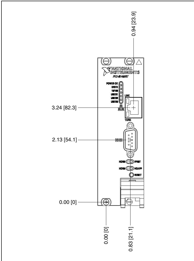
Figure C-1. PXI-8145RT Front Panel Layout and Dimensions
